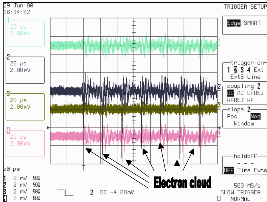
Figure 1 : Electron cloud peaks on channel 2, spaced 23\mu S. No electron cloud detected on the other pick-ups.
