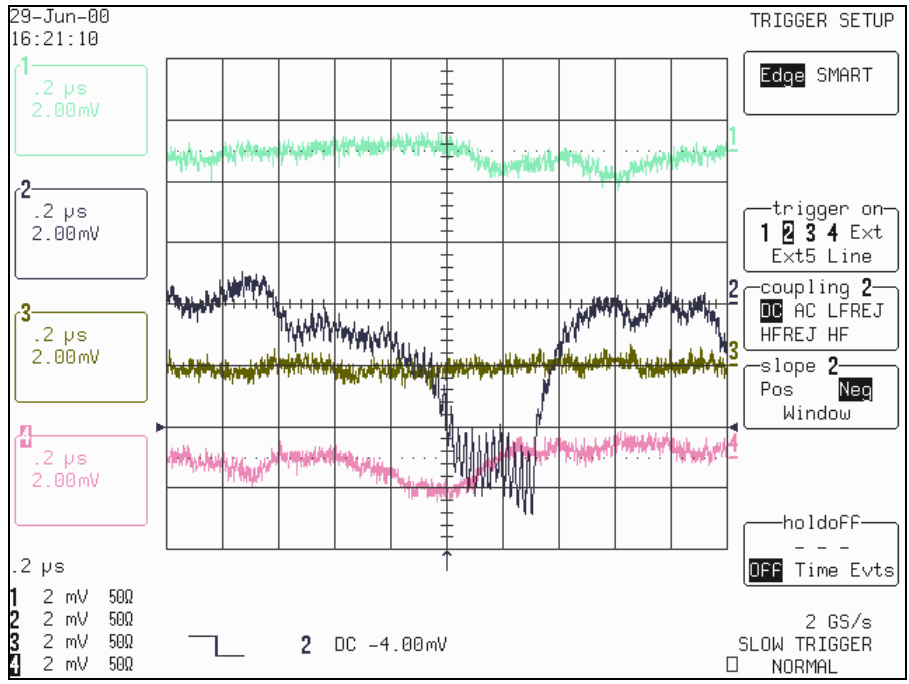
Figure 3 : Detail of electron cloud (channel 2). No electron cloud on the other pick-ups.
