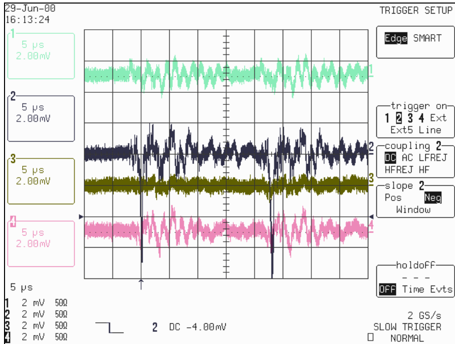
Figure 2 : Electron cloud peaks (channel 2), no electron cloud on other pick-ups.
