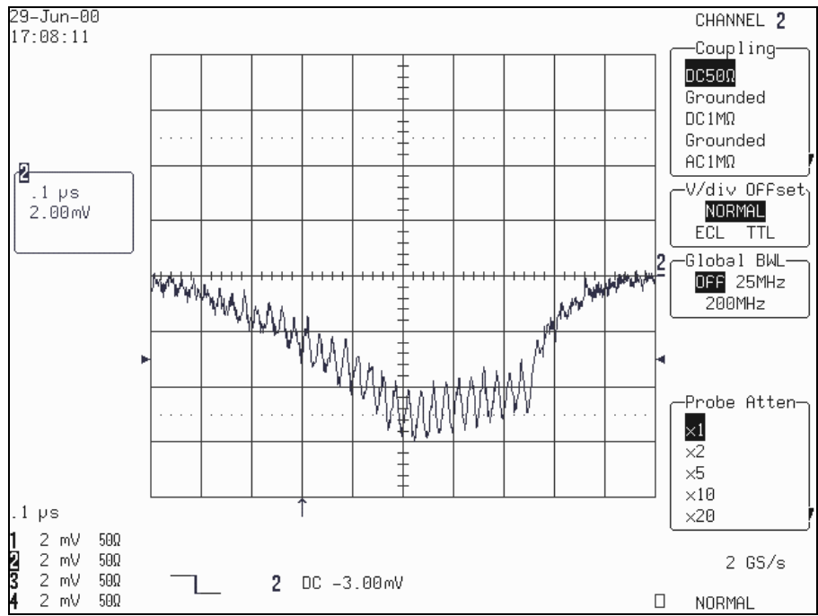
Figure 4 : Detail of electron cloud peak.
