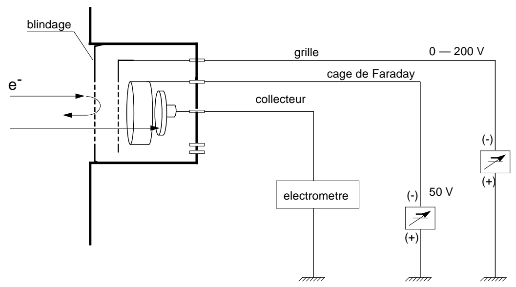
principle of energy analysis
